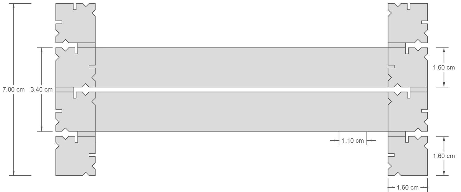
Top view
