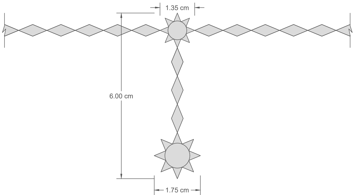
Front view
